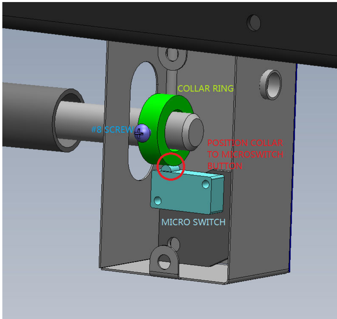
Diagram #12: SAFETYBAR COLLAR INSTALLATION (Optional)
