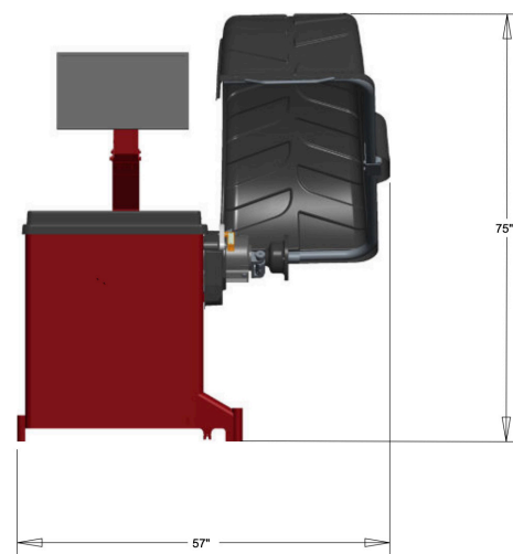
Wheel Balancer Dimensions without wheel lift
