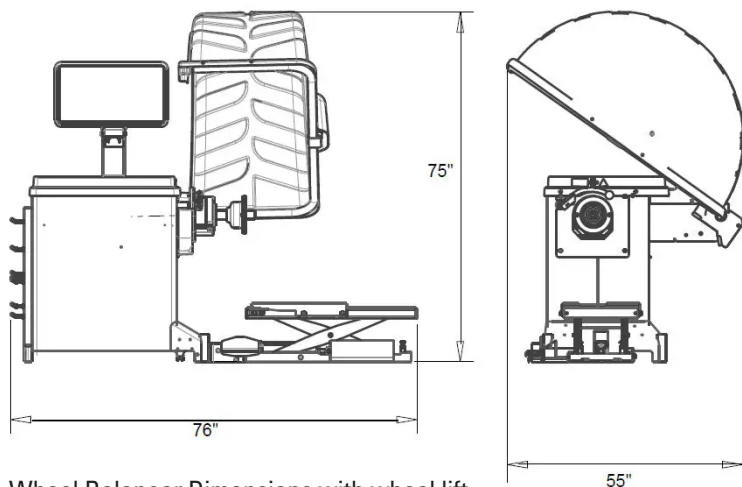
Wheel Balancer Dimensions with wheel lift
